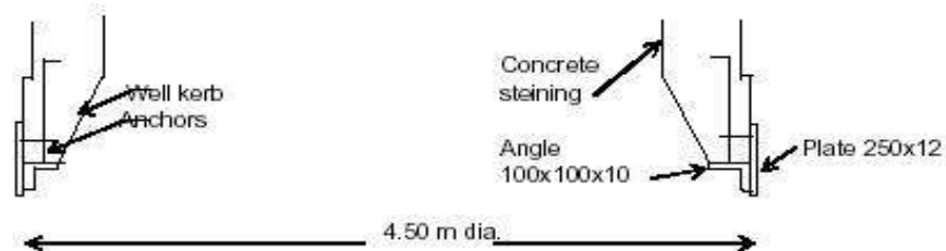
DETAILS OF FOUNDATION WELL CUTTING EDGE
